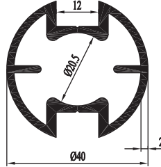
62 4244 00 0.988 kg/m
