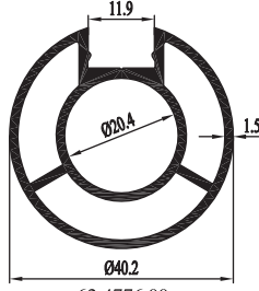
62 4776 00 0.879 kg/m
