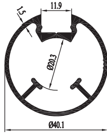
62 5082 00 0.696 kg/m
