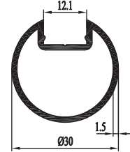
62 5804 00 0.414 kg/m
