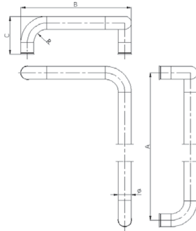
Baston Kollar
