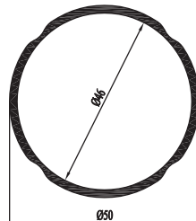
62 5623 20 0.769 kg/m.
