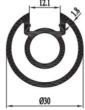
62 5241 00 0.414 kg/m
